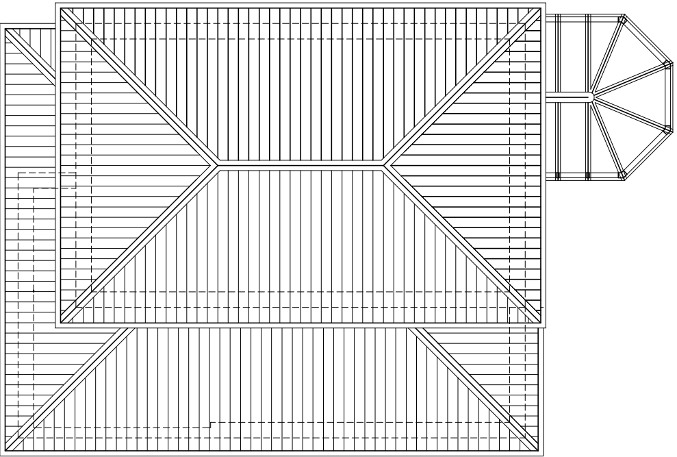
Existing Roof Plan 1:100
