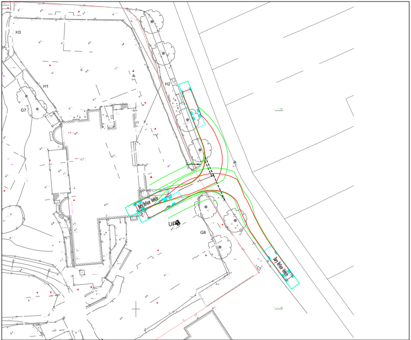
REFUSE TRACKING - LEFT IN/LEFT OUT (SCALE 1:1000)
