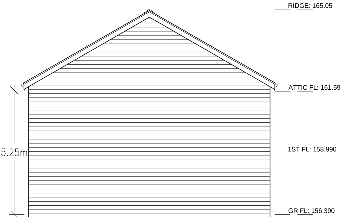
PROPOSED SIDE/NORTH ELEVATION (1:100)
