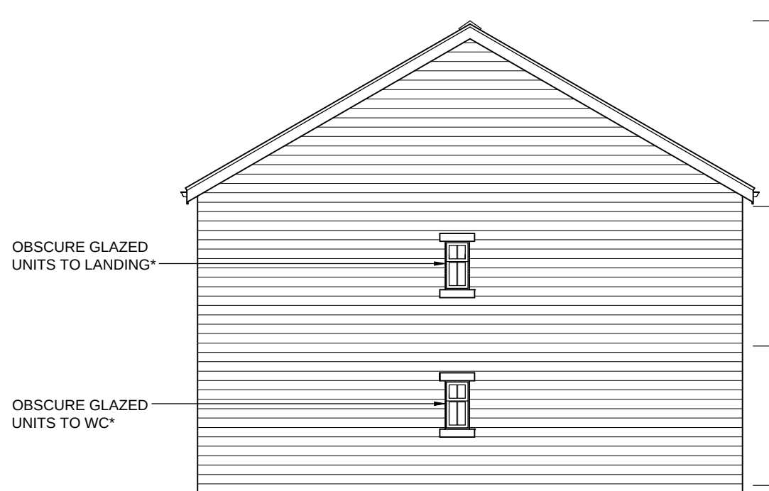
PROPOSED SIDE/SOUTH ELEVATION (1:100)
