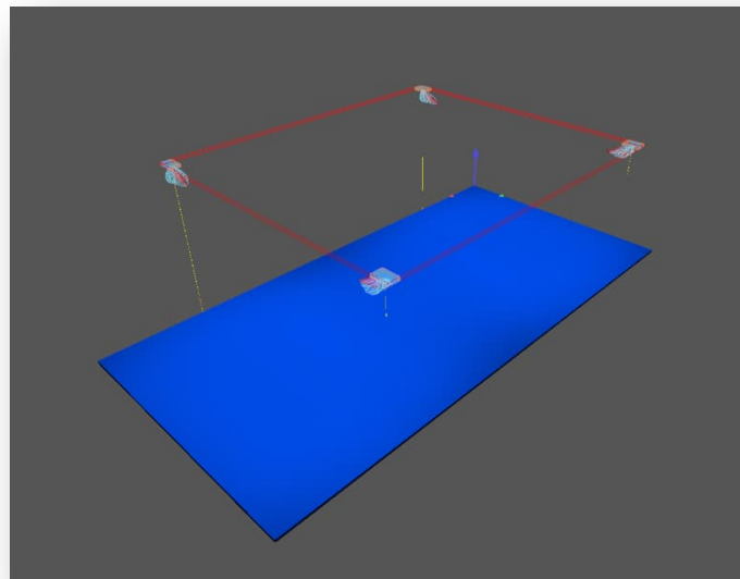
Figure 7.11: Luminaire 3D model, 6m from ground level and 0° tilt facing downward.
