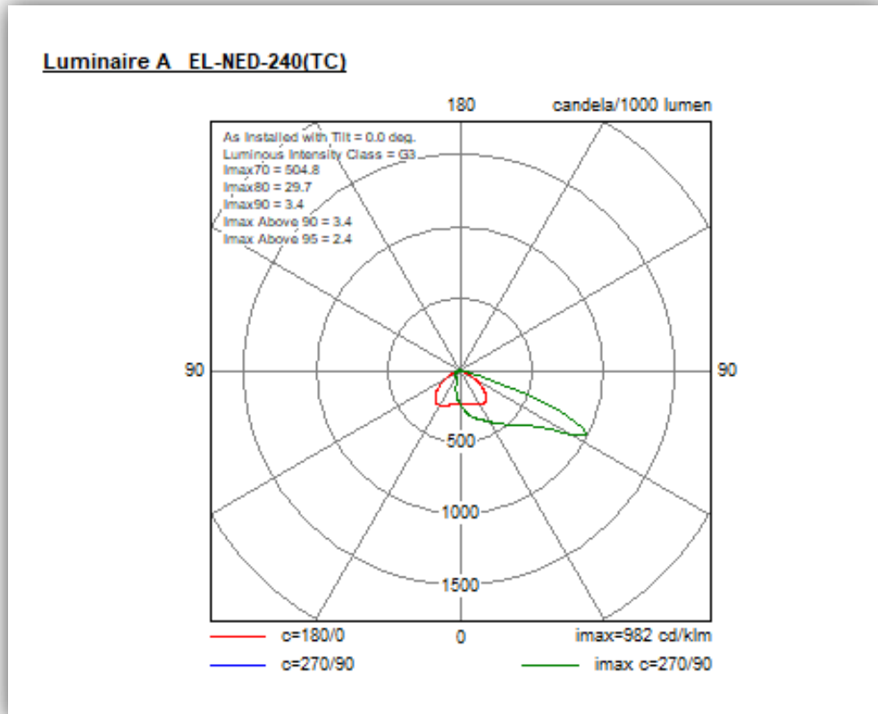
Figure 7.10: Polar diagram for EL NED 240 (TC) floodlight
