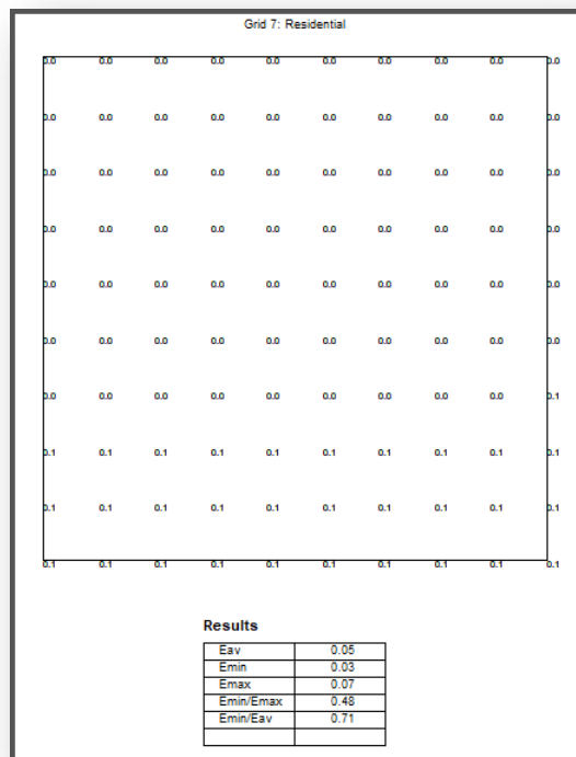
Figure 7.4: Residential vertical calculation results
