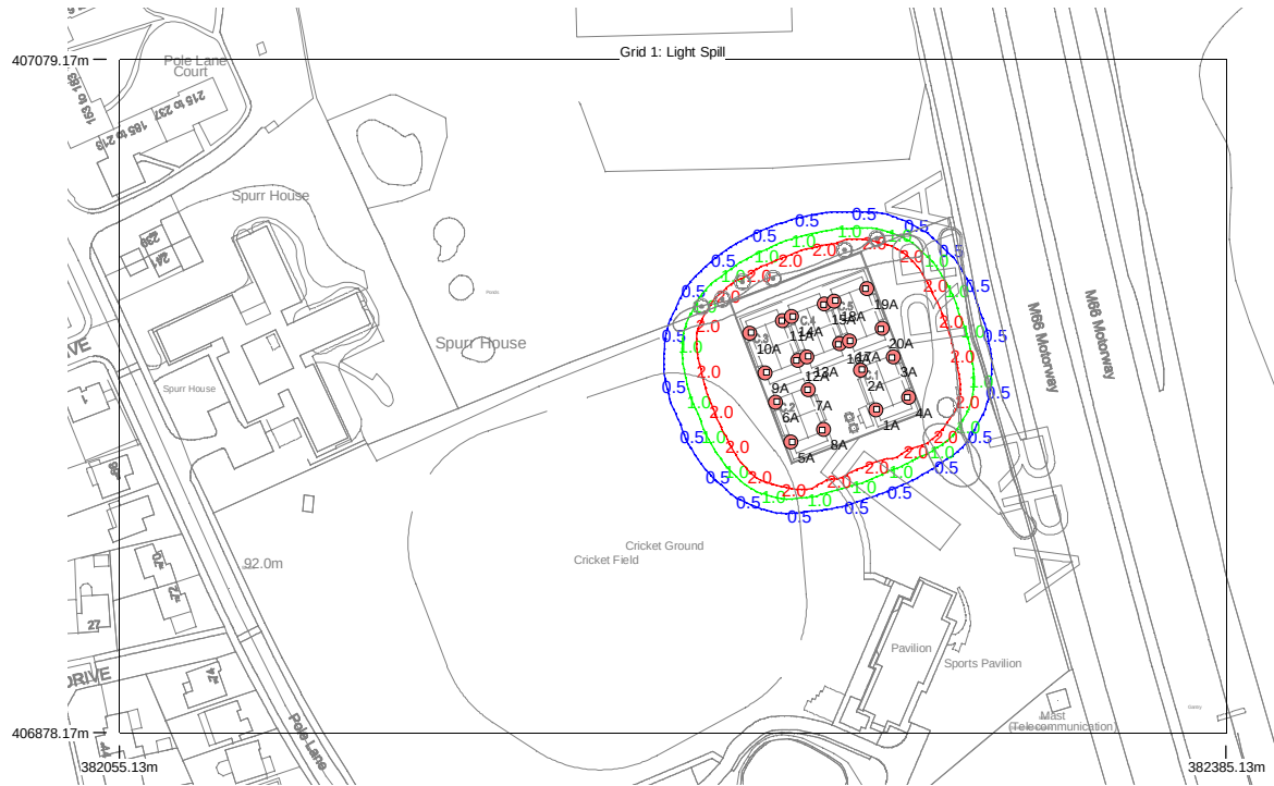
Grid 1: Light Spill
