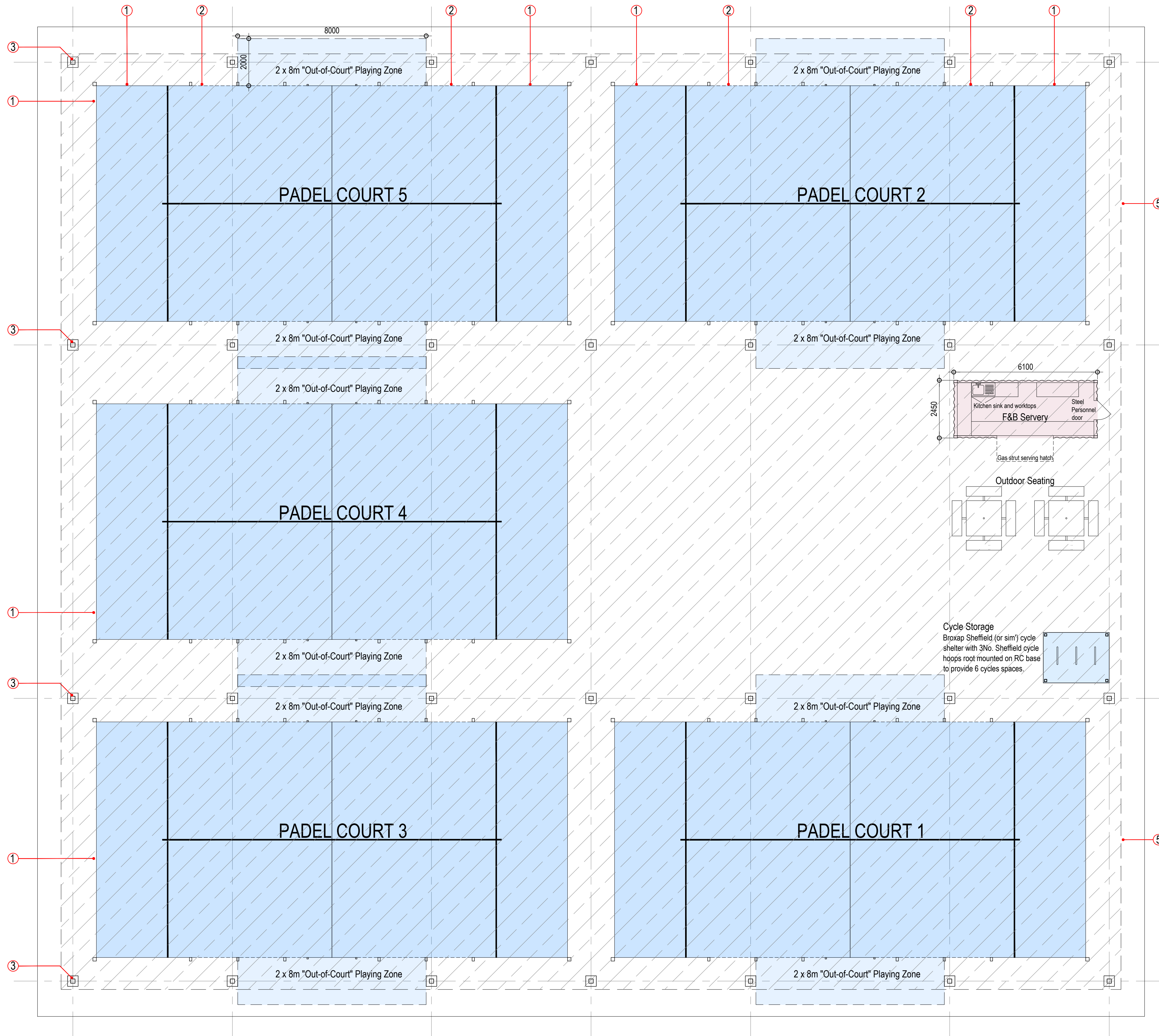
PROPOSED PADEL COURTS G.A. PLAN 1:100@A1
