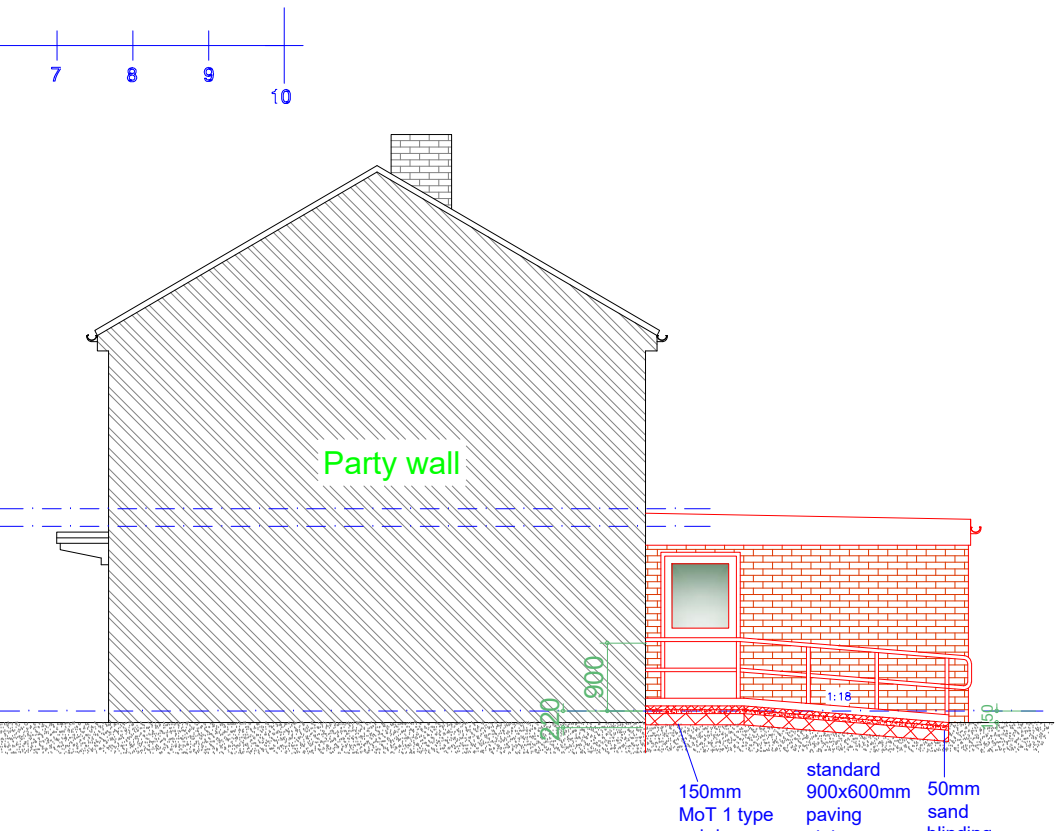
Proposed R/H Side Party Wall Elevation Scale 1:100
