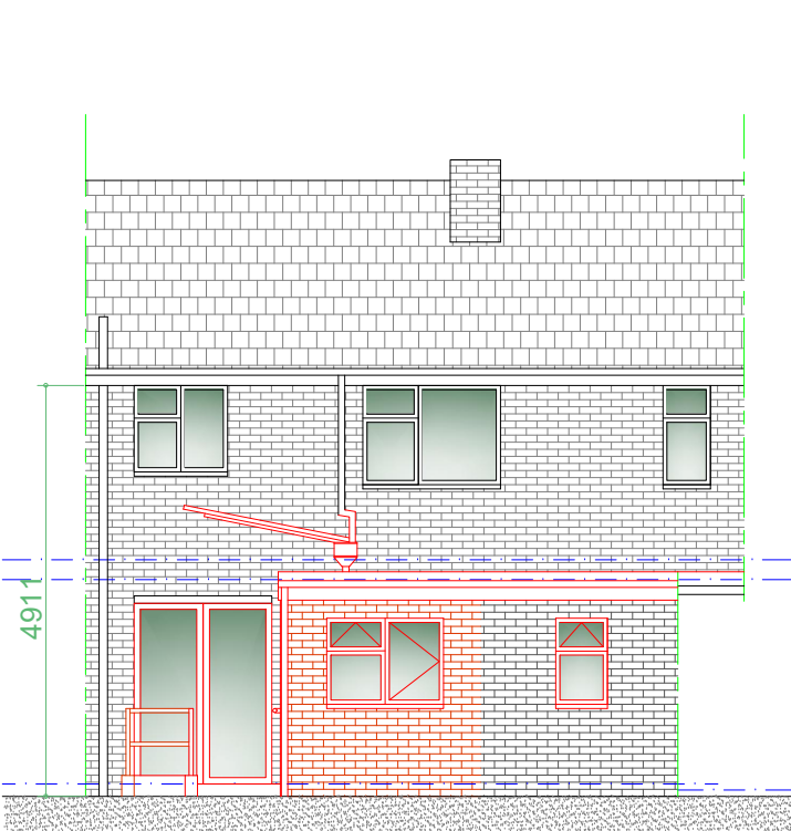
Proposed Rear Elevation (Outbuilding) Scale 1:100
