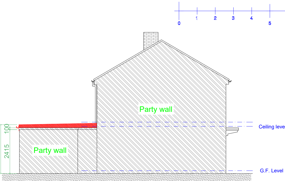
Proposed L/H Side Party Wall Elevation Scale 1:100
