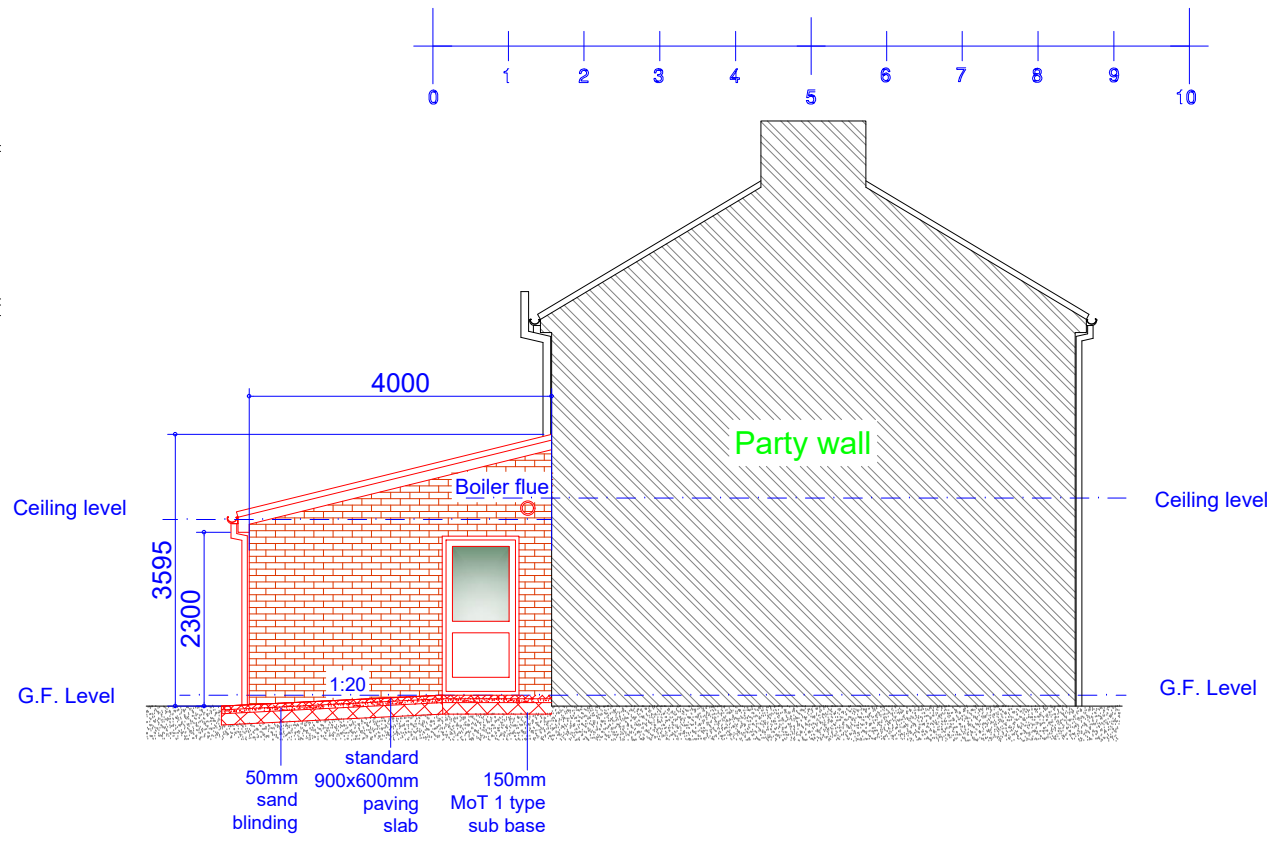
Proposed R/H Side Party Wall Elevation Scale 1:100
