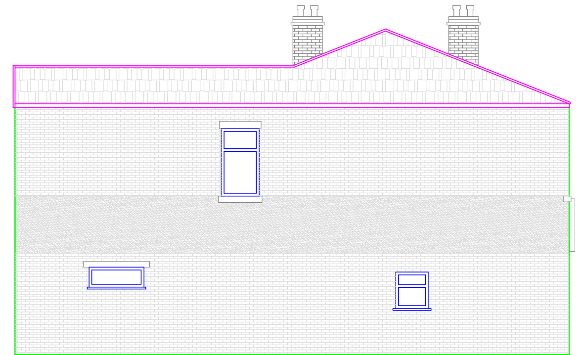
(West) Existing Side Elevation of no. 110
