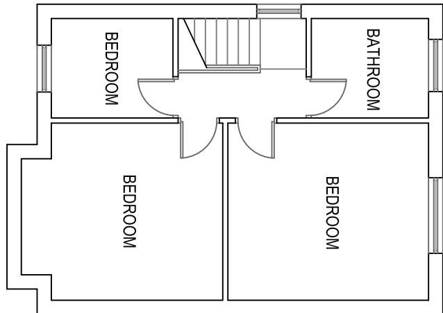
EXISTING FF PLAN 1:100
