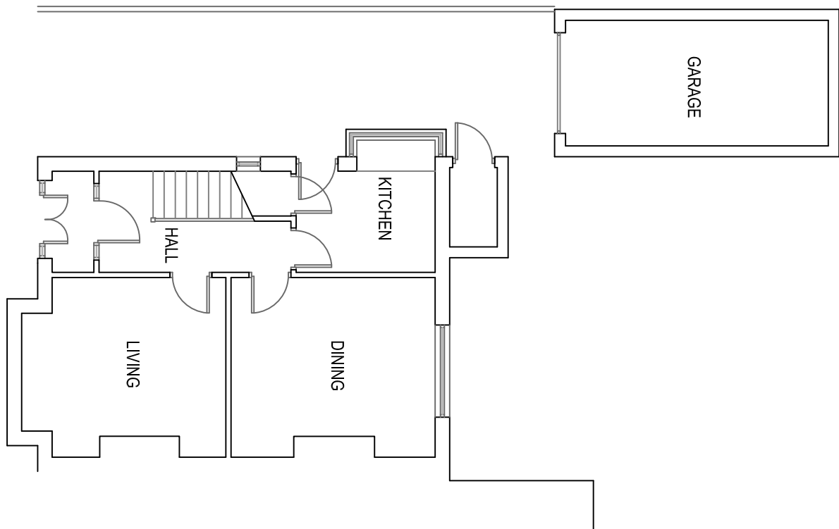
EXISTING GF PLAN 1:100
