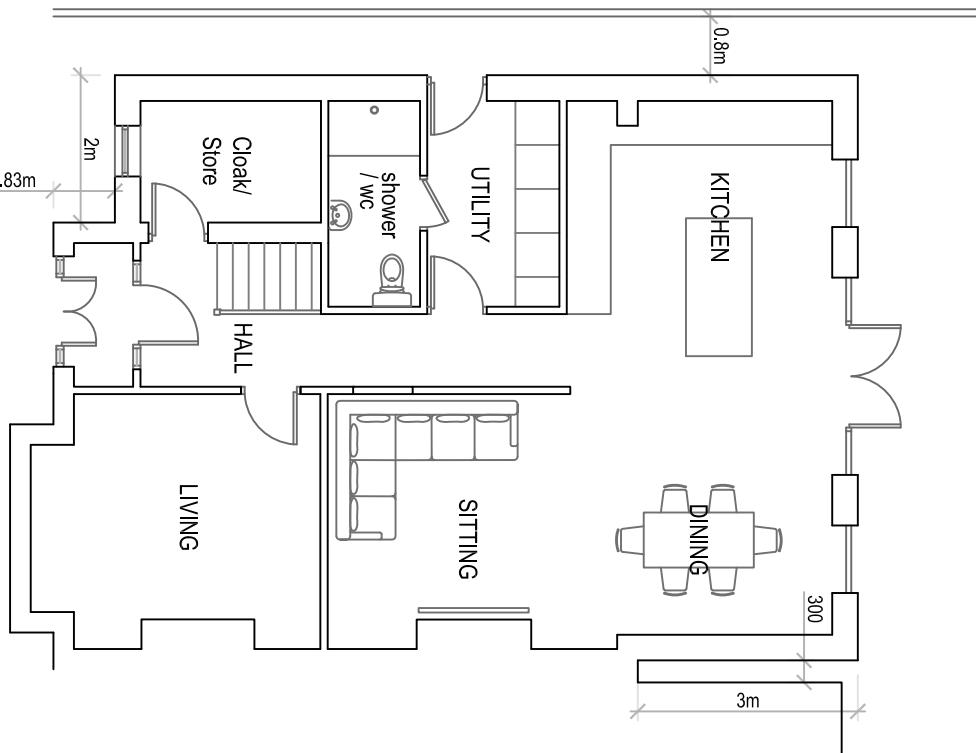
PROPOSED GF PLAN 1:100
