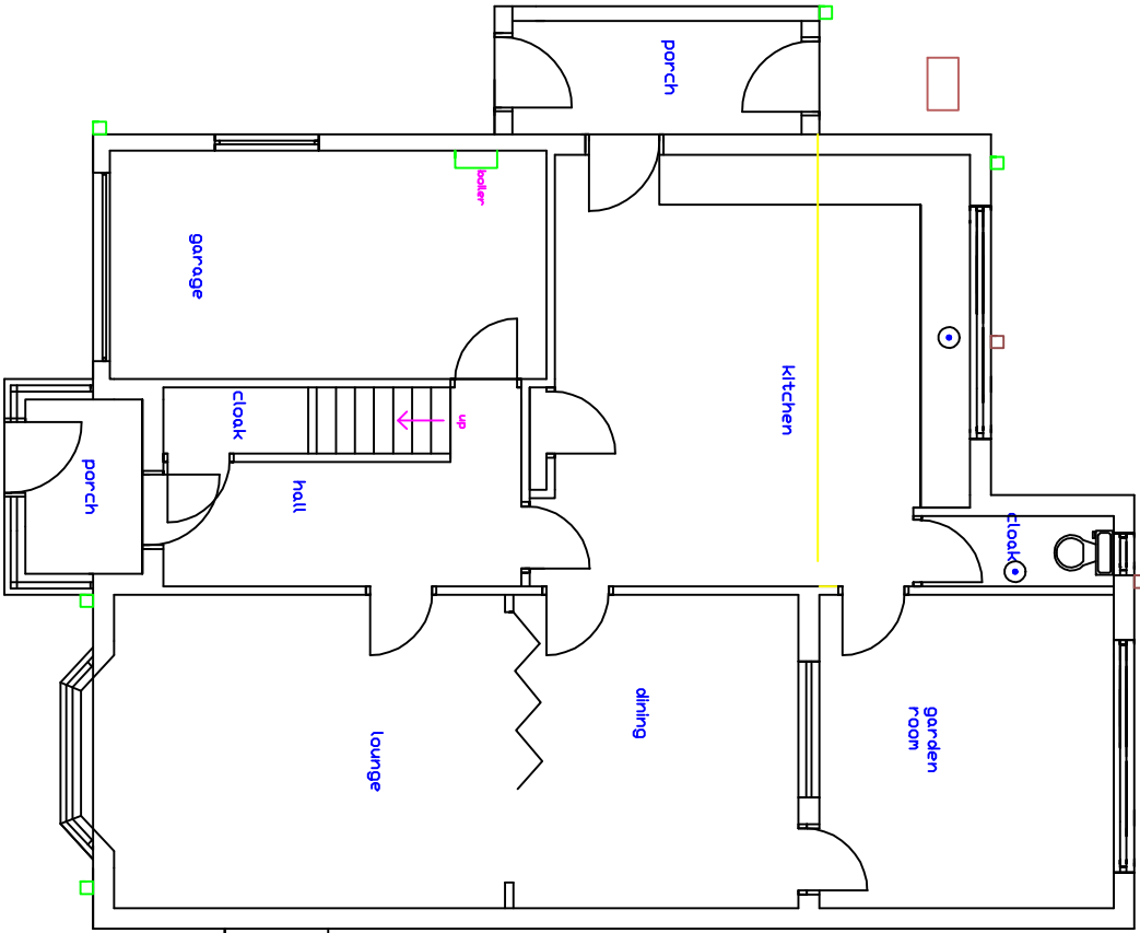
EXISTING GROUND FLOOR LAYOUT 1:100
