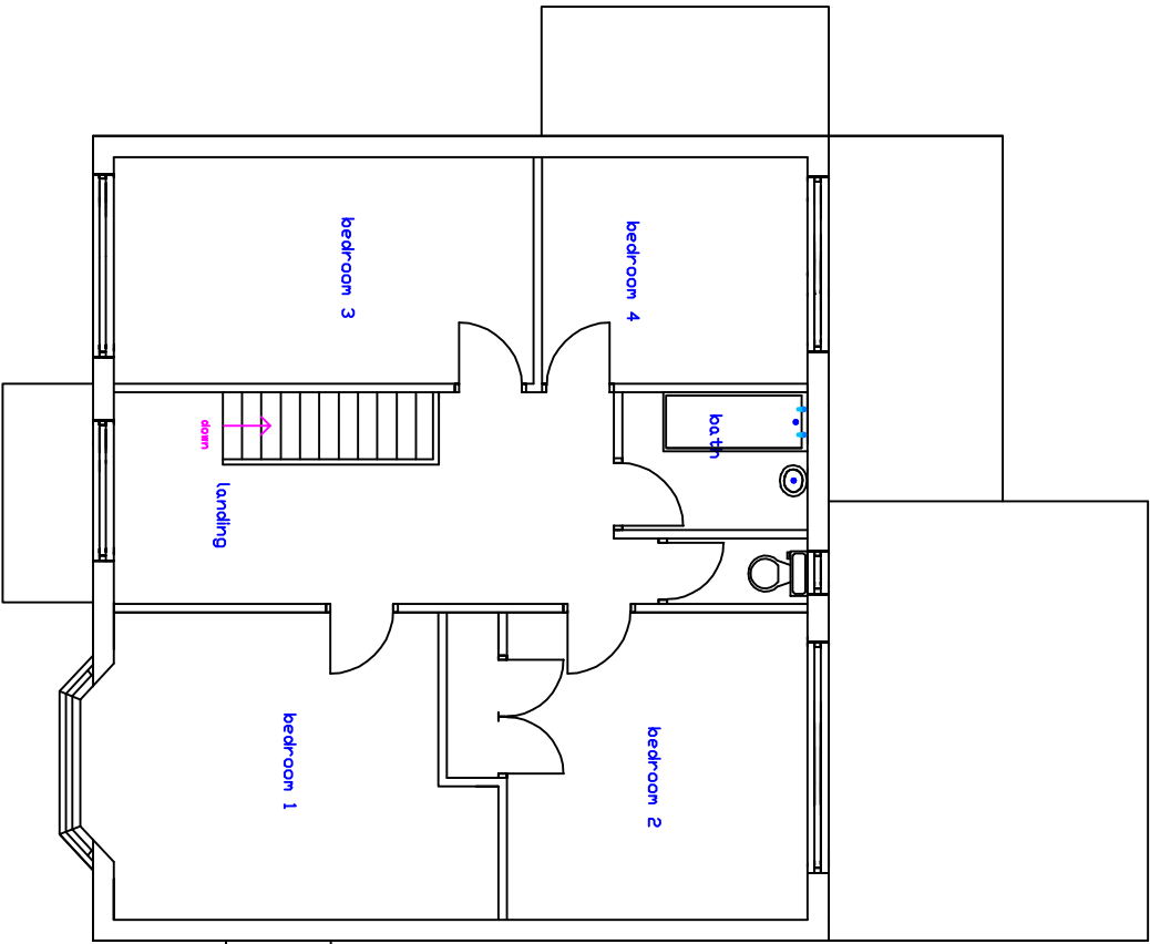
EXISTING FIRST FLOOR LAYOUT 1:100
