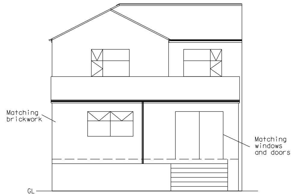
REAR ELEVATION
