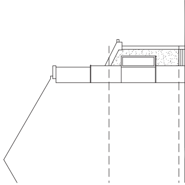
PROPOSED RETURN ELEVATION
