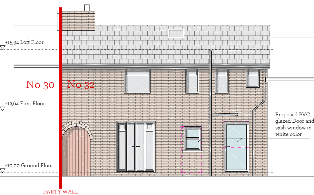
Proposed Elevation South
