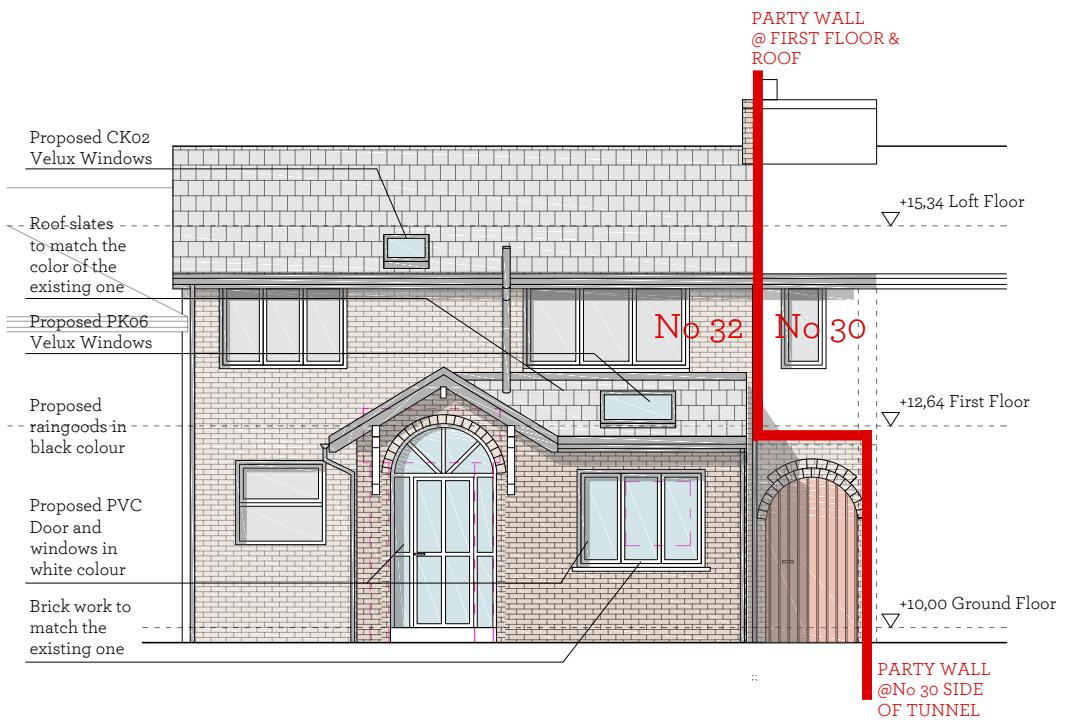
Proposed Elevation North
