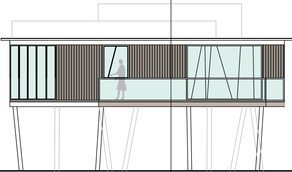
Elevation to North 0 1m 5m
