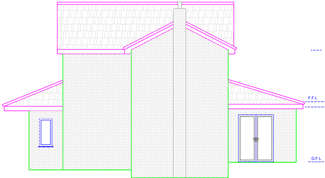
EXISTING SIDE ELEVATION (SOUTH WEST)
