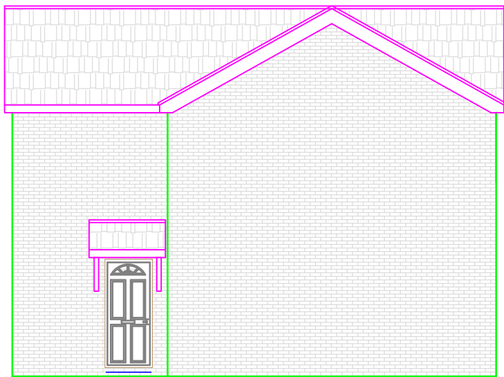
Existing Side Elevation (EAST)
