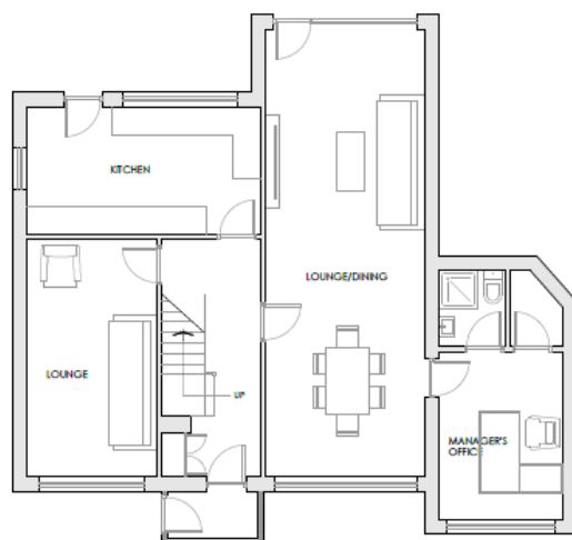
PROPOSED GROUND FLOOR PLAN 1:50
