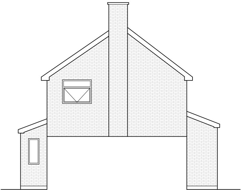
PROPOSED SIDE ELEVATION 1:100 @ A3
