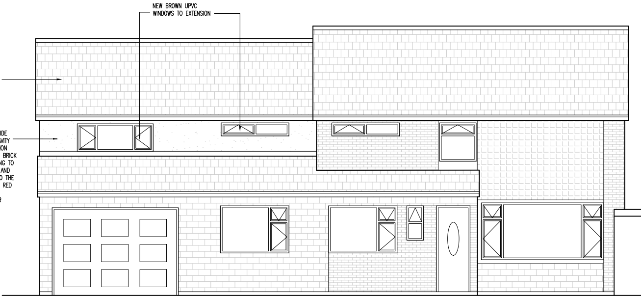
PROPOSED FRONT ELEVATION 1:100 @ A3
