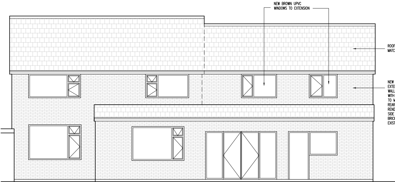
PROPOSED REAR ELEVATION 1:100 @ A3
