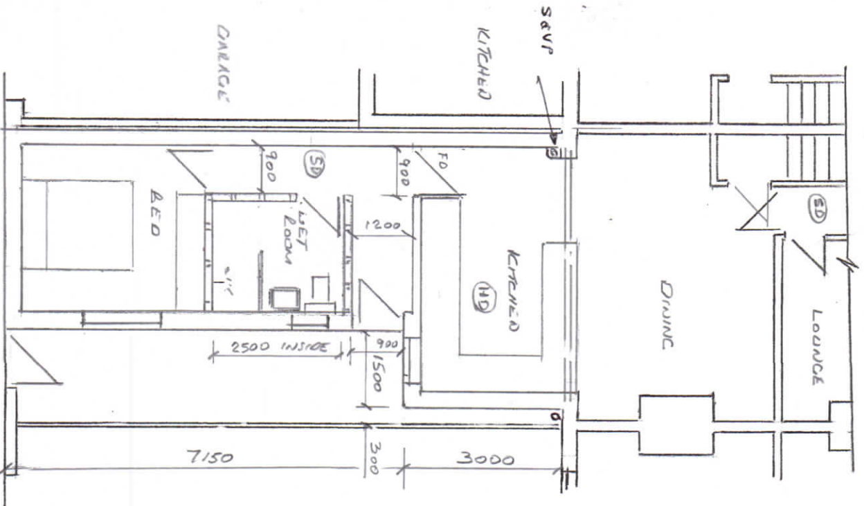
PROPOSED REAR EXTENSION
