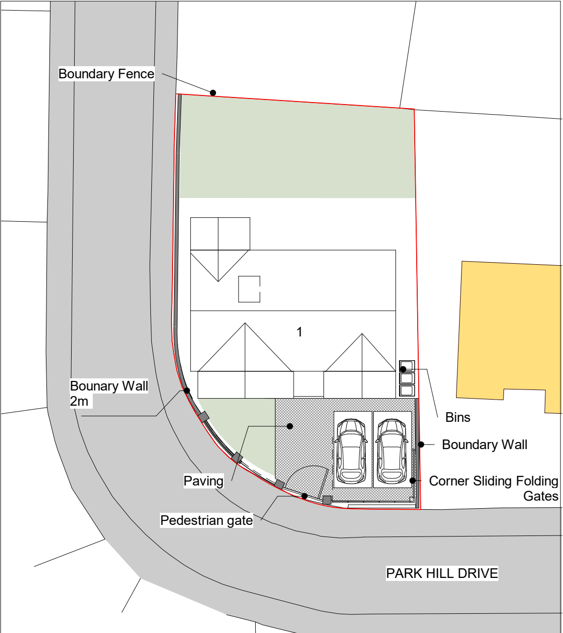
2. Site Proposed Parking 1 : 250
