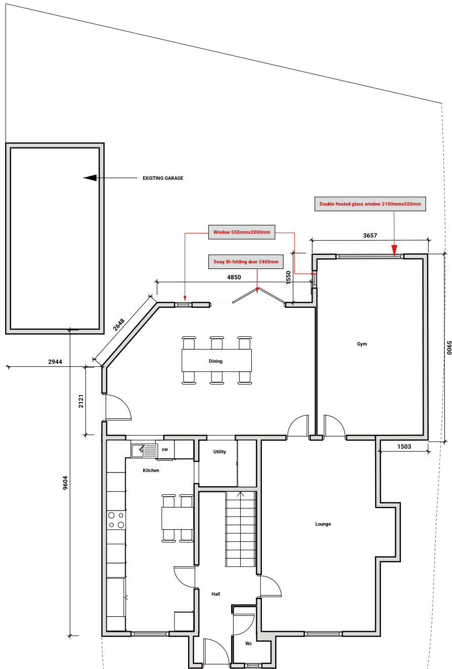
Proposed Ground Floor Scale 1:50
