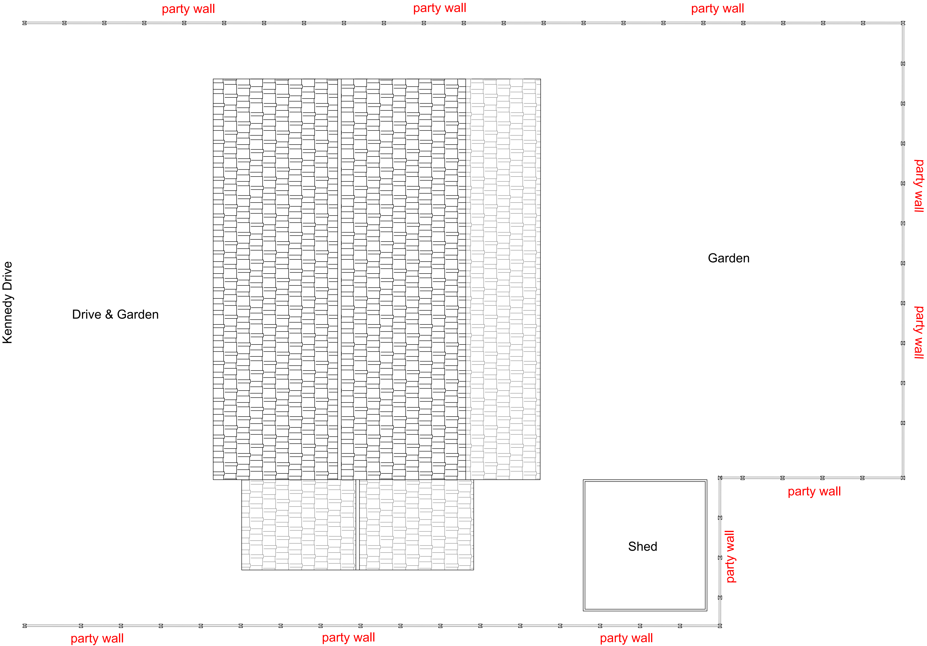
EXISTING GROUND FLOOR PLAN 1:50 @ A1
