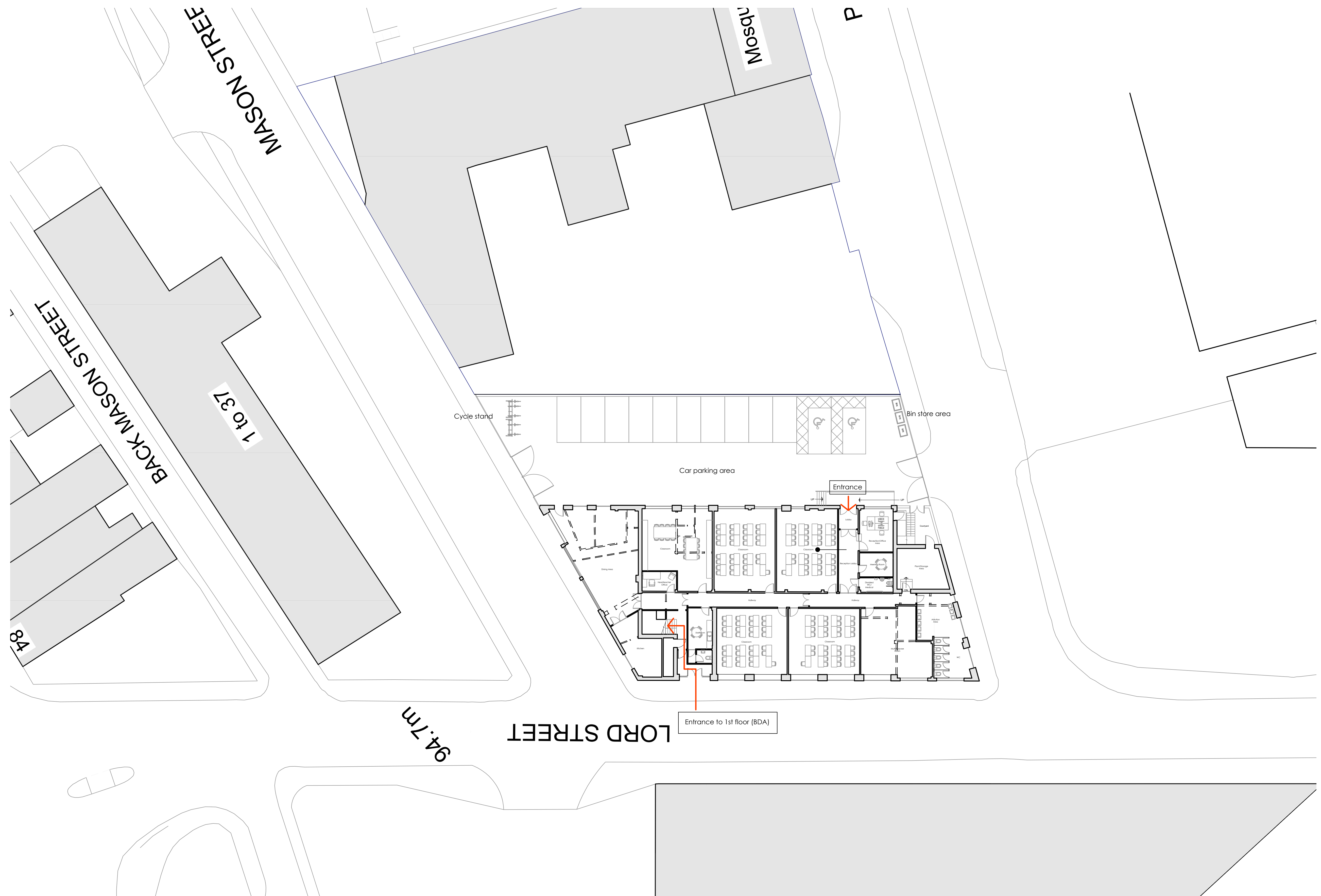
PROPOSED SITE LAYOUT PLAN 1:200
