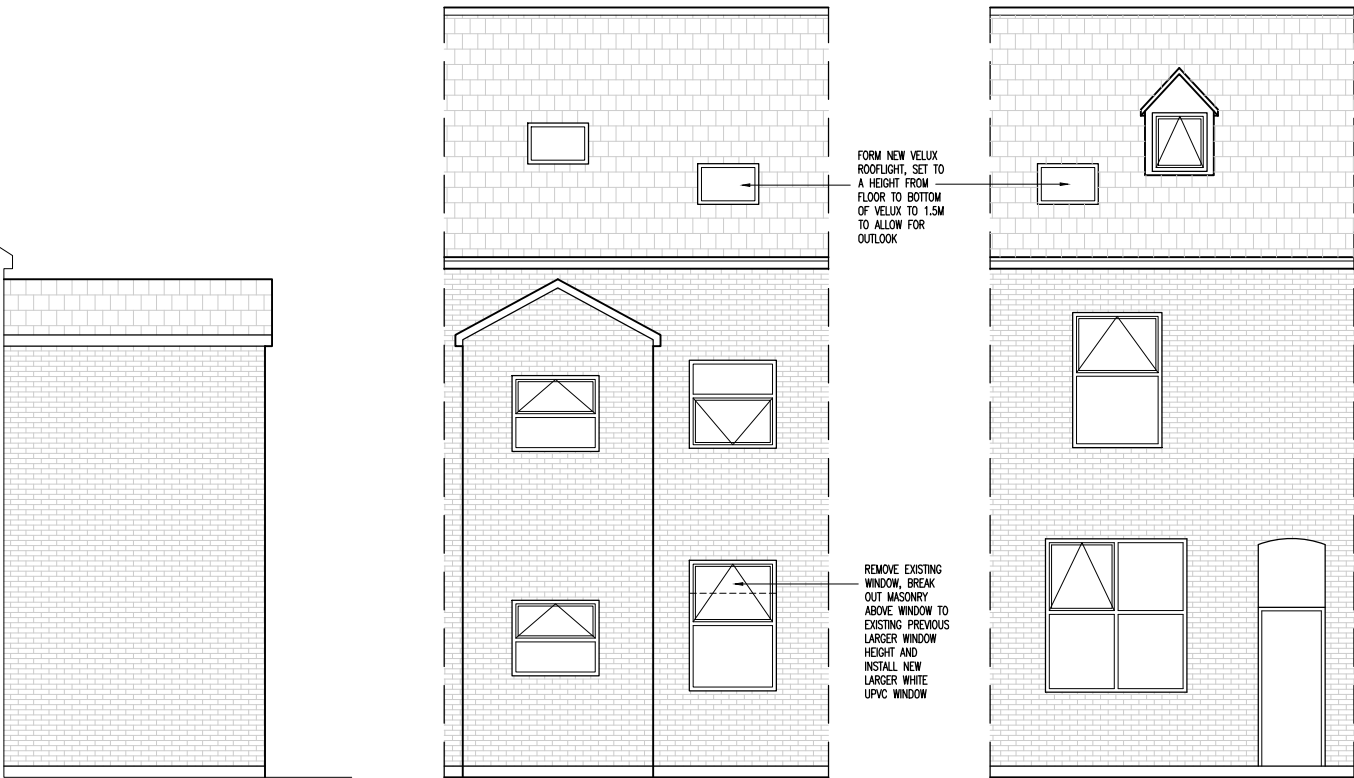
PROPOSED SIDE/REAR ELEVATION 1:100 @ A3
