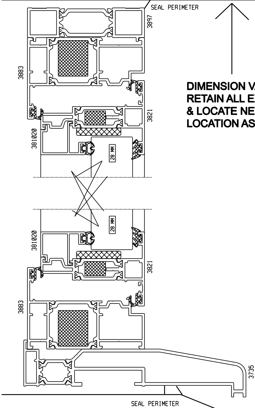
A - A HEAD & CILL SECTIONS AA
