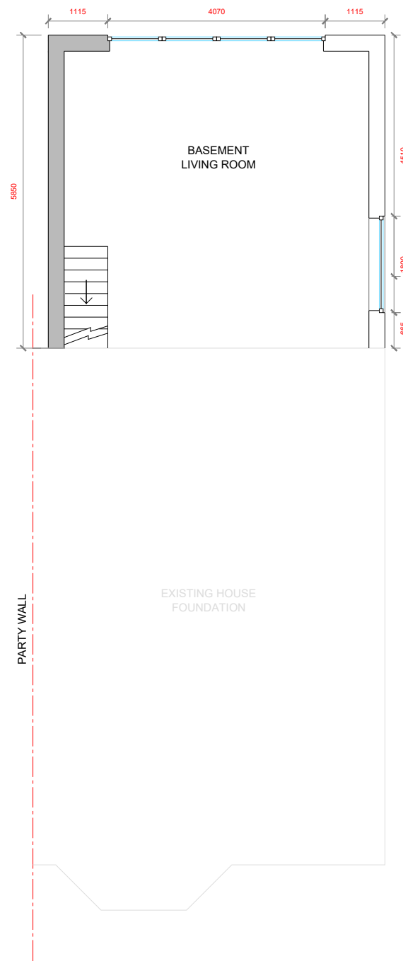
BASEMENT PLAN
