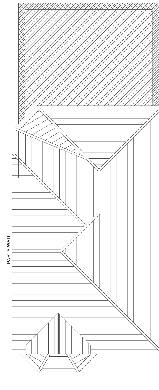
ROOF PLAN
