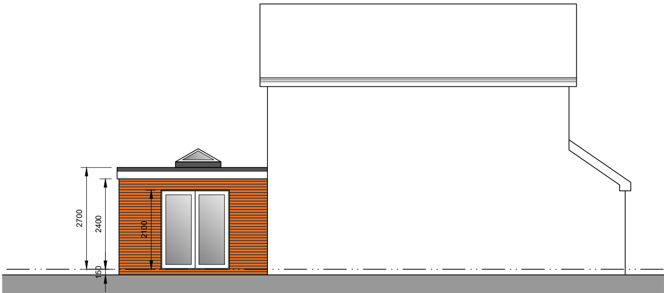
North East Facing Side Elevation
