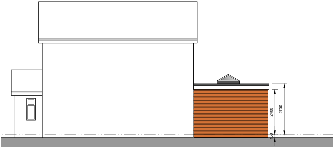
South West Facing Side Elevation
