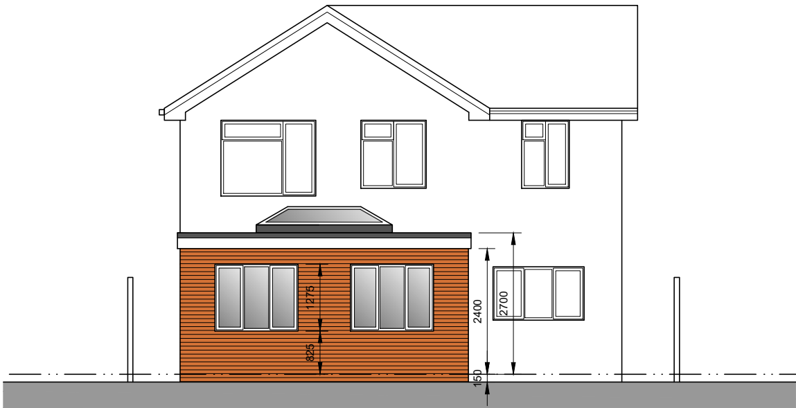
South East Facing Rear Elevation
