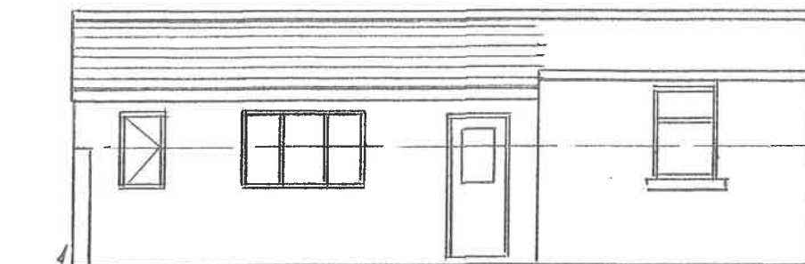
PROPOSED SIDE ELEVATION
