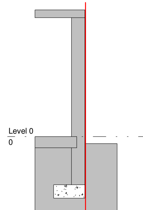
3 Section between 33 and 35 1 : 50
