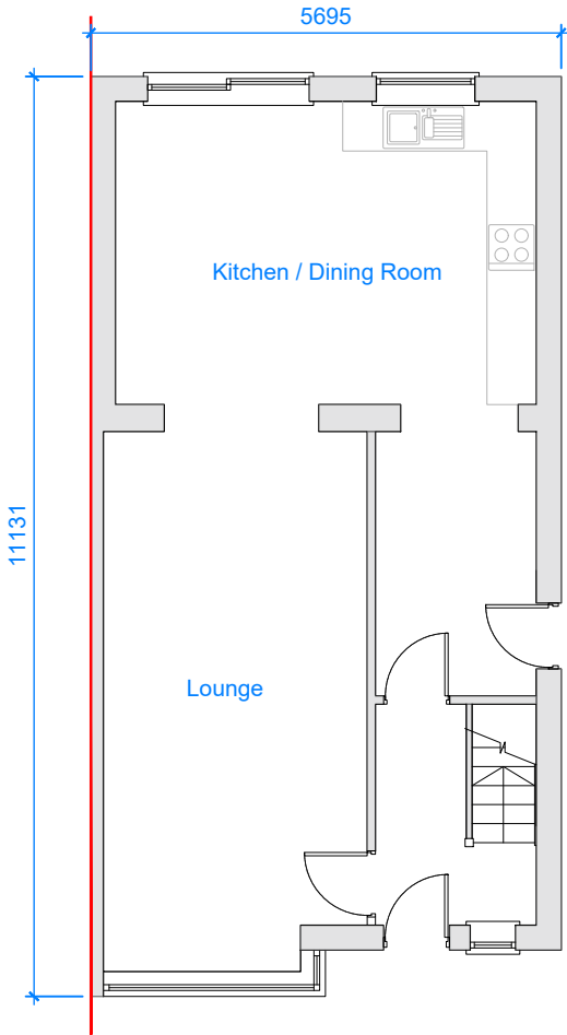
EXISTING GROUND FLOOR @1:50
