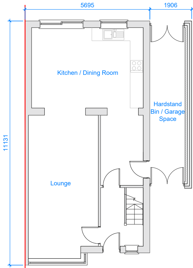
PROPOSED GROUND FLOOR @1:50
