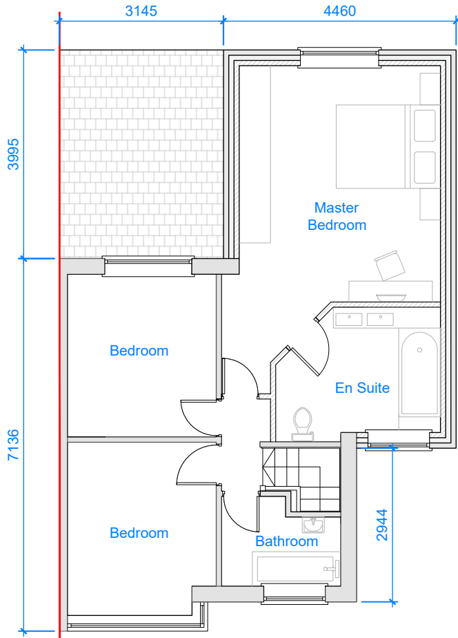
PROPOSED FIRST FLOOR @1:50
