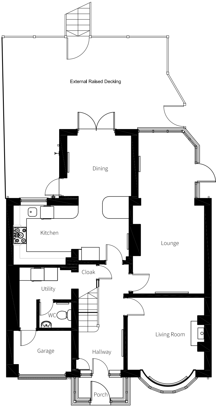
Existing Ground Floor Plan 1:100 / A3
