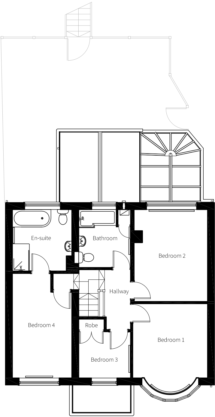
Existing First Floor Plan 1:100 / A3
