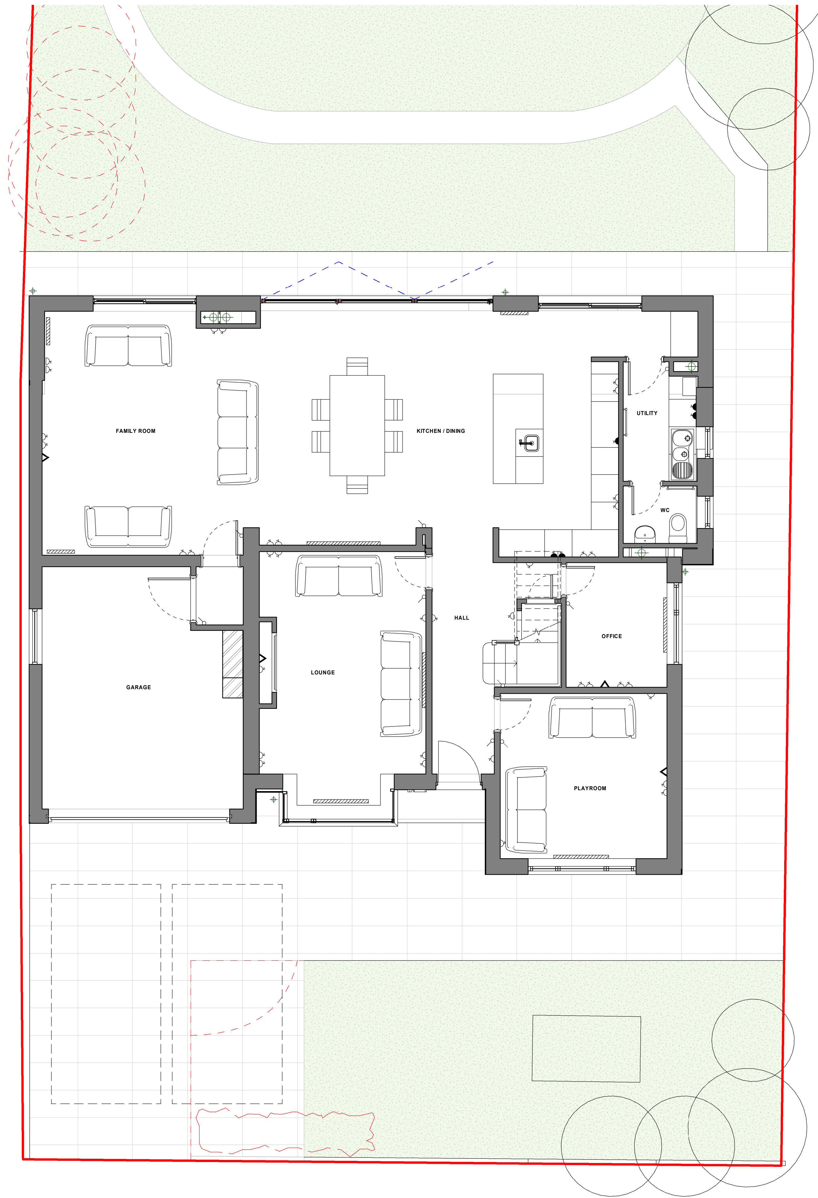
1 Level 0 - Proposed GA Plan 1 : 50
