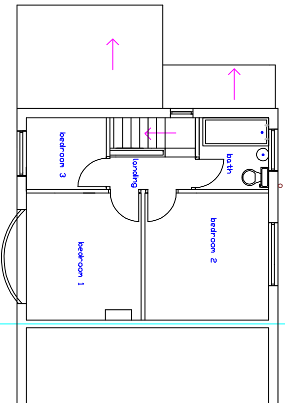
EXISTING FIRST FLOOR 1:100
