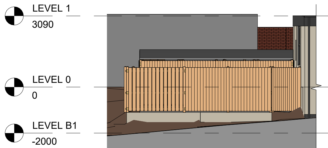
2 Front - Proposed Bin and Bike 1 : 100
