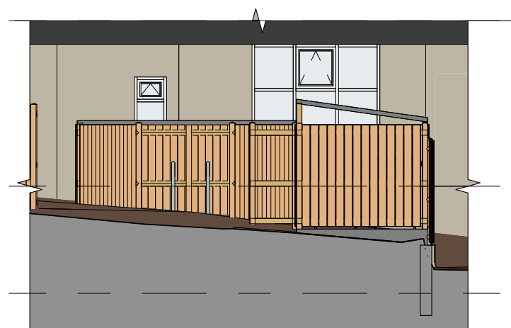
3 Left Side - Proposed Bin and Bike 1 : 100
