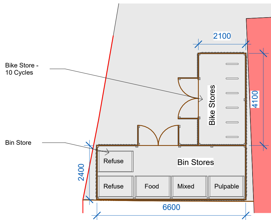
1 Site - Proposed Bin and Bike Stores 1 : 100
