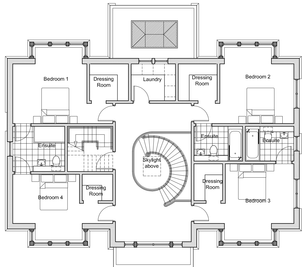
Proposed House 2 1/F Plan 1:100
