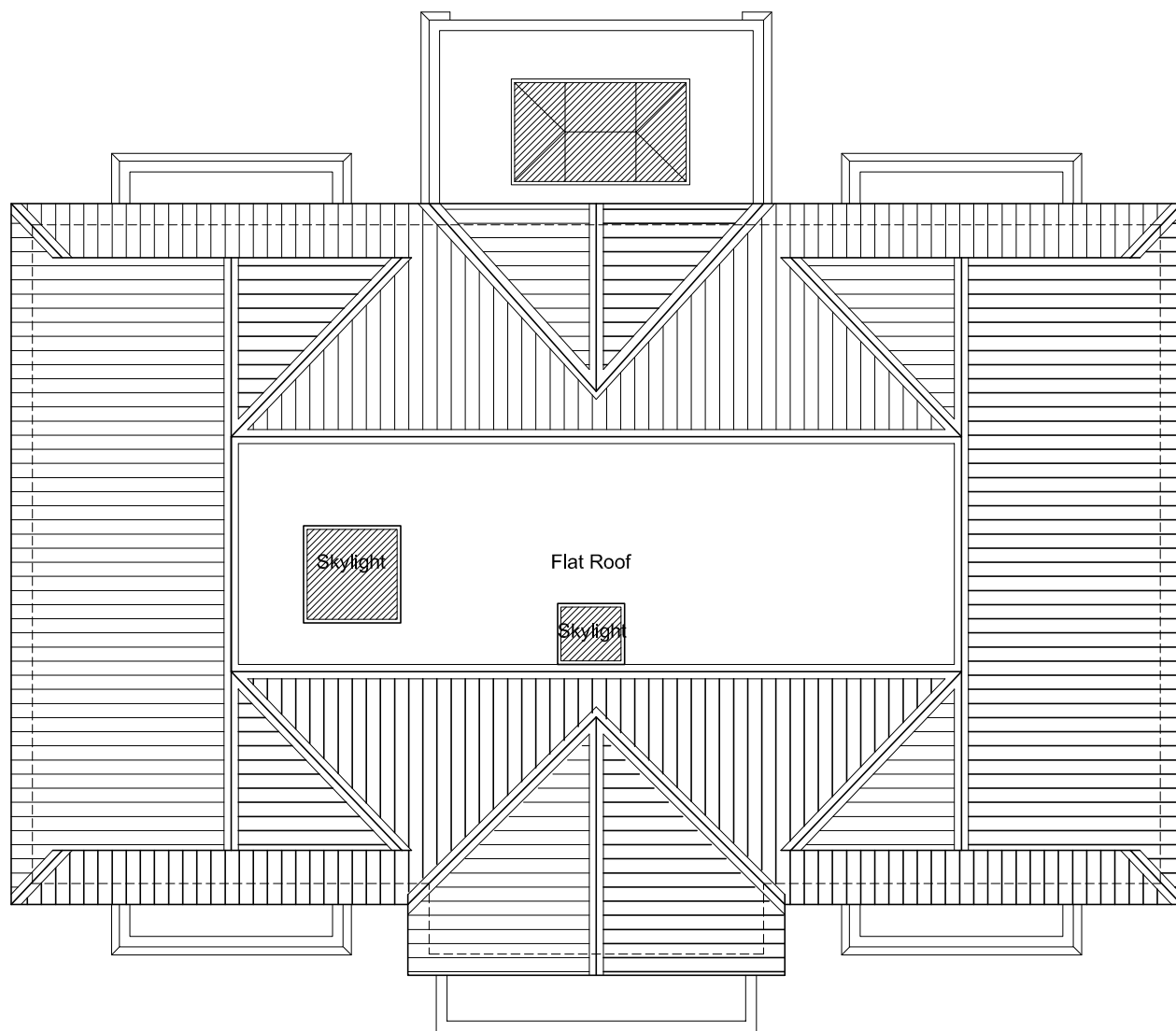
Proposed House 2 Roof Plan 1:100
