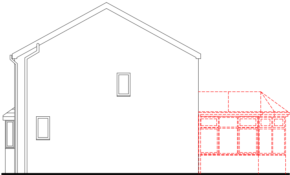
Side Elevation
