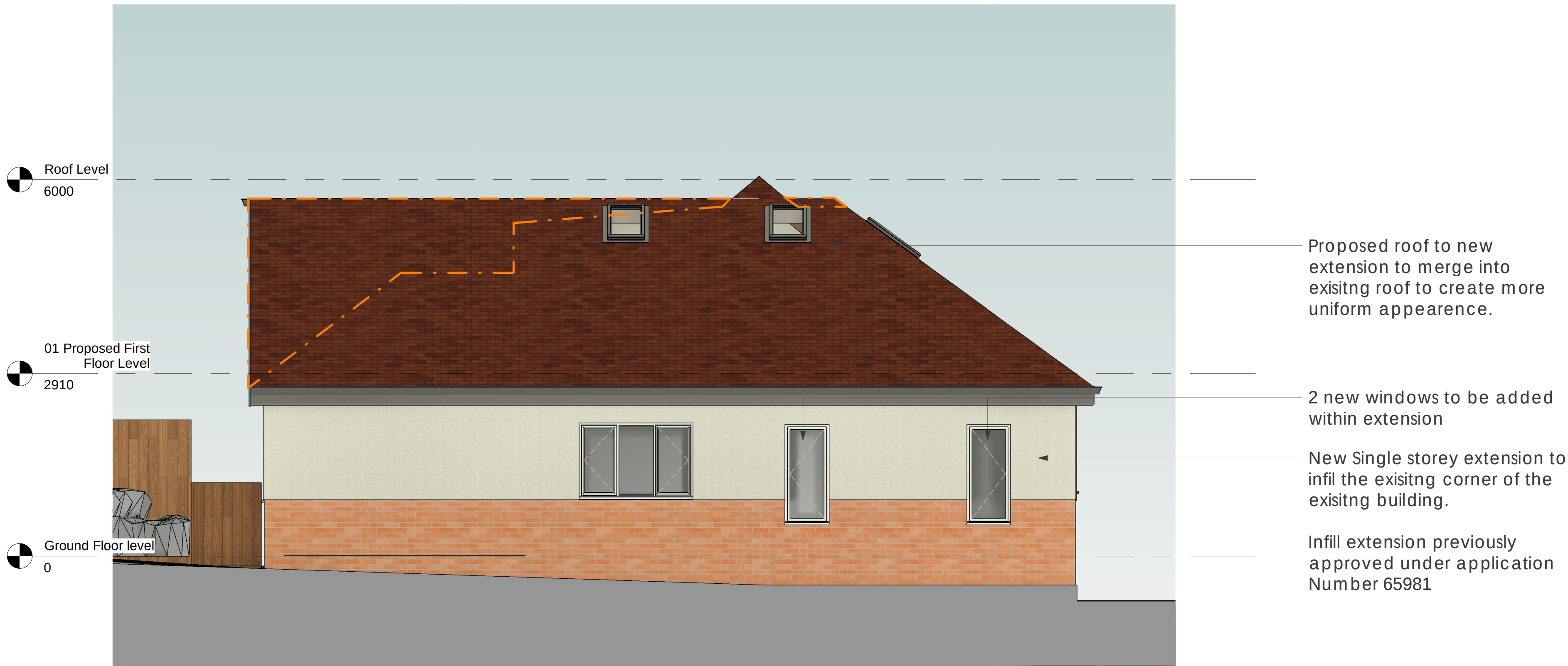
Proposed LHS Elevation Scale: 1 : 50
