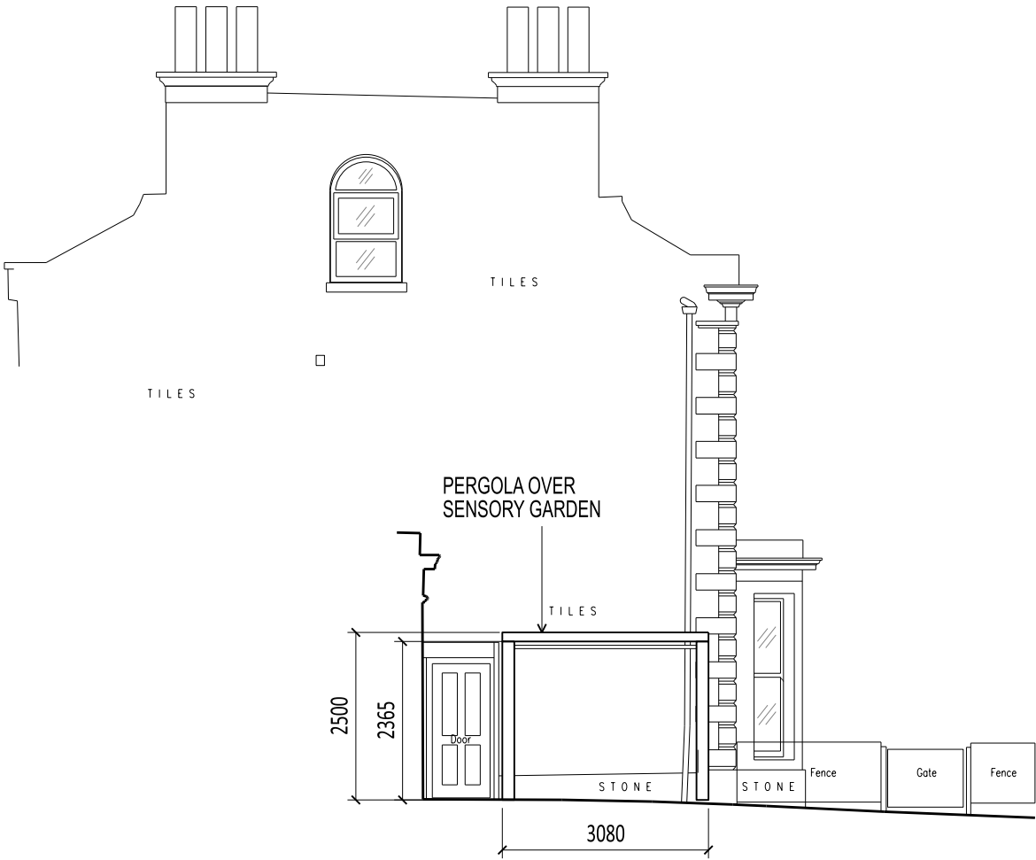
SIDE ELEVATION A
