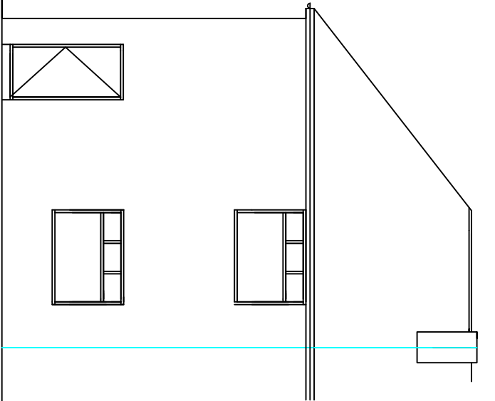
EXISTING REAR VIEW 1:100
