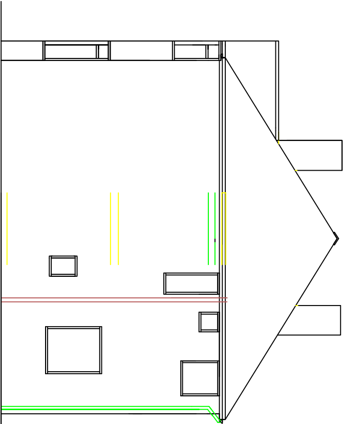
EXISTING SIDE VIEW A 1:100
