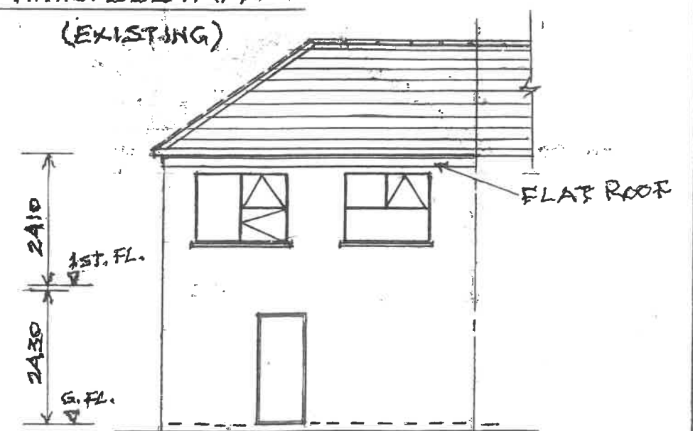
REAR ELEVATION
