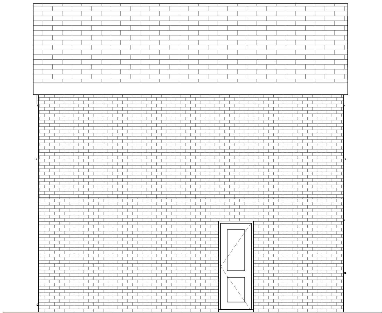
2 East Existing 1 : 50
