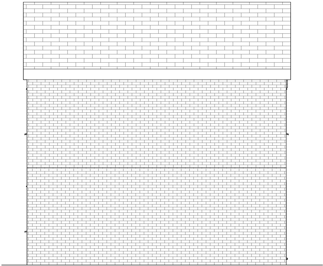
3 West Existing 1 : 50
