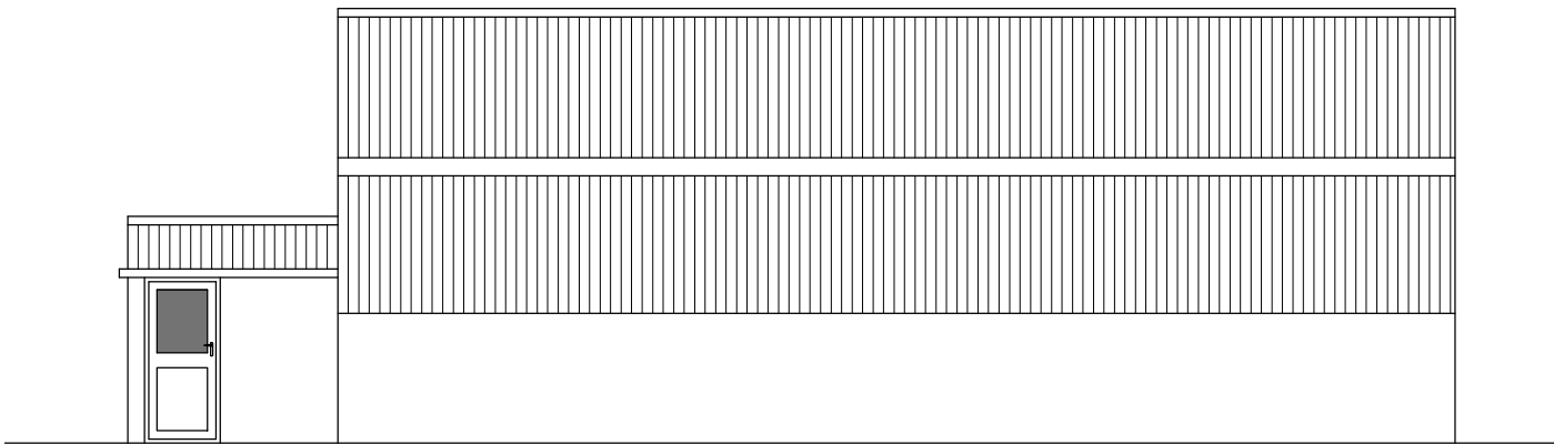
EXISTING FRONT ELEVATION (EAST)
