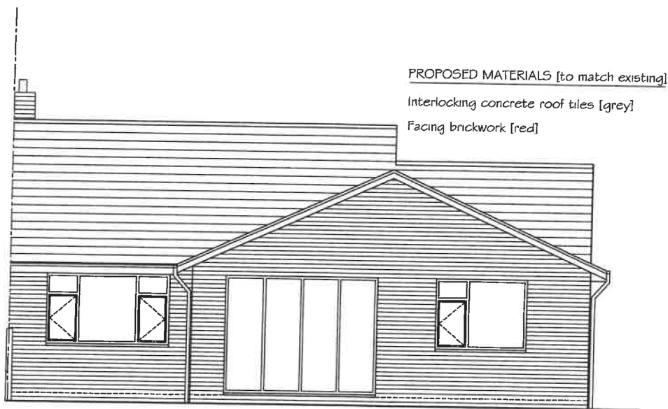
PROPOSED NORTH EAST ELEVATION 1:100 @ A4
