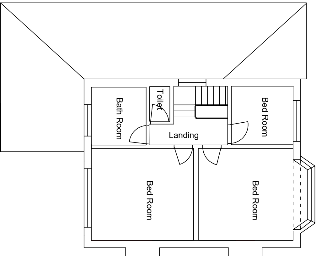
1st Floor
