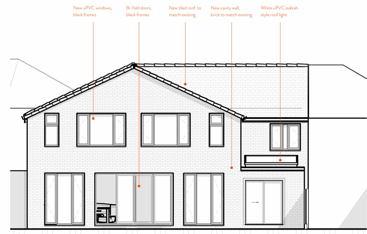
8 West - Proposed 1 : 100
