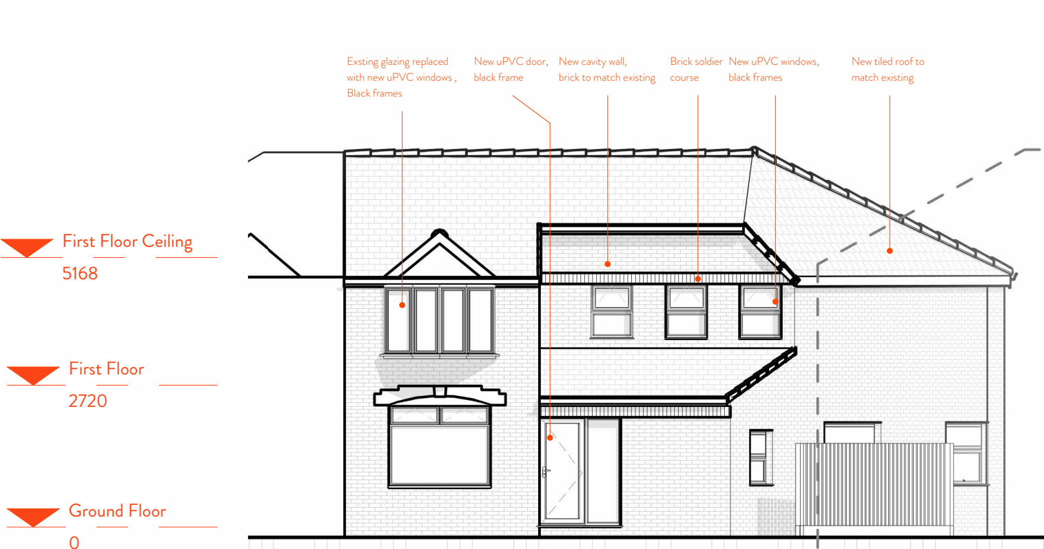
5 East - Proposed 1 : 100
