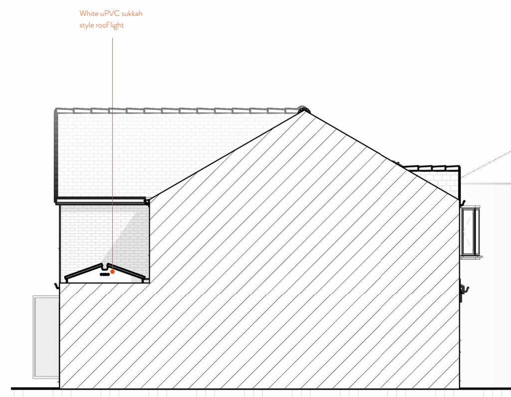
7 South - Proposed 1 : 100
