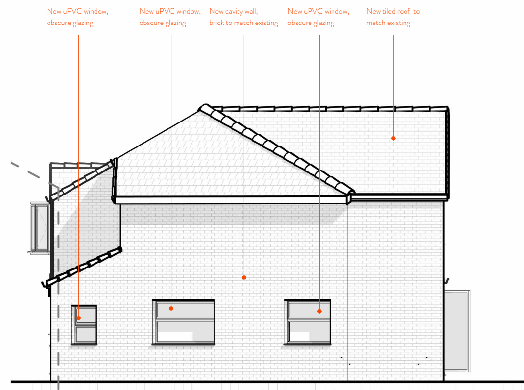
6 North - Proposed 1 : 100
