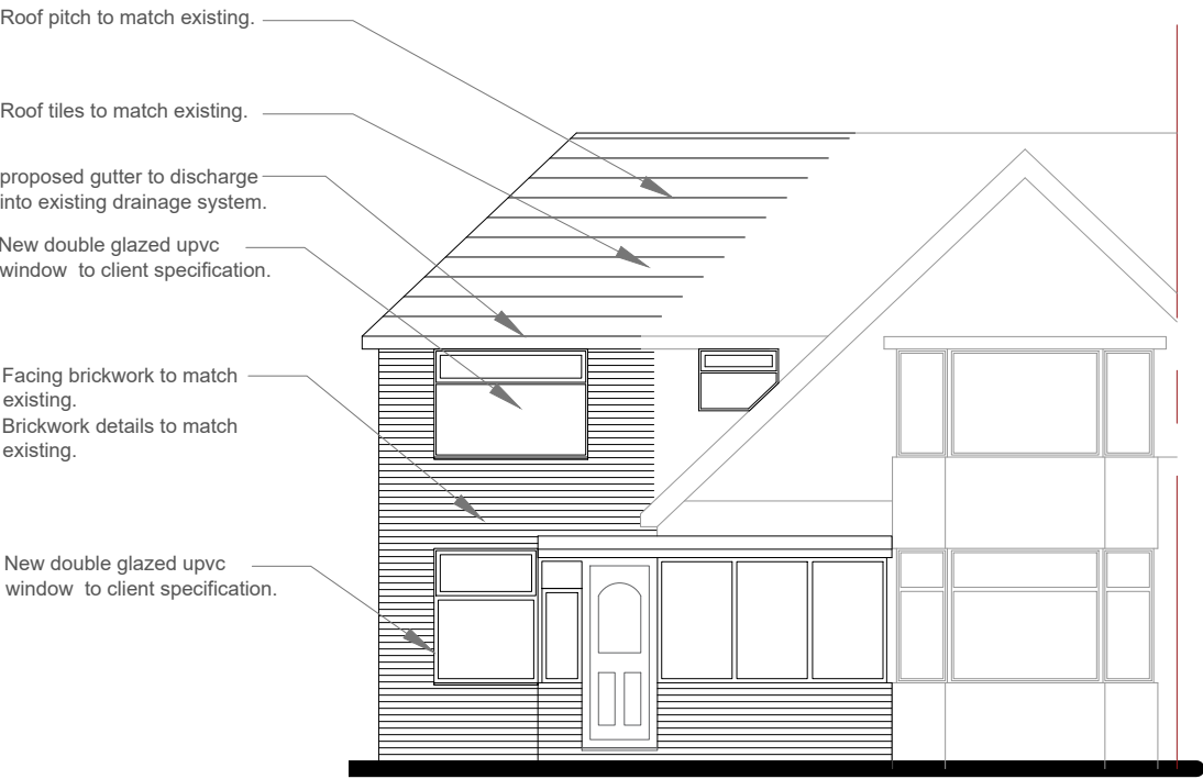
FRONT ELEVATION
