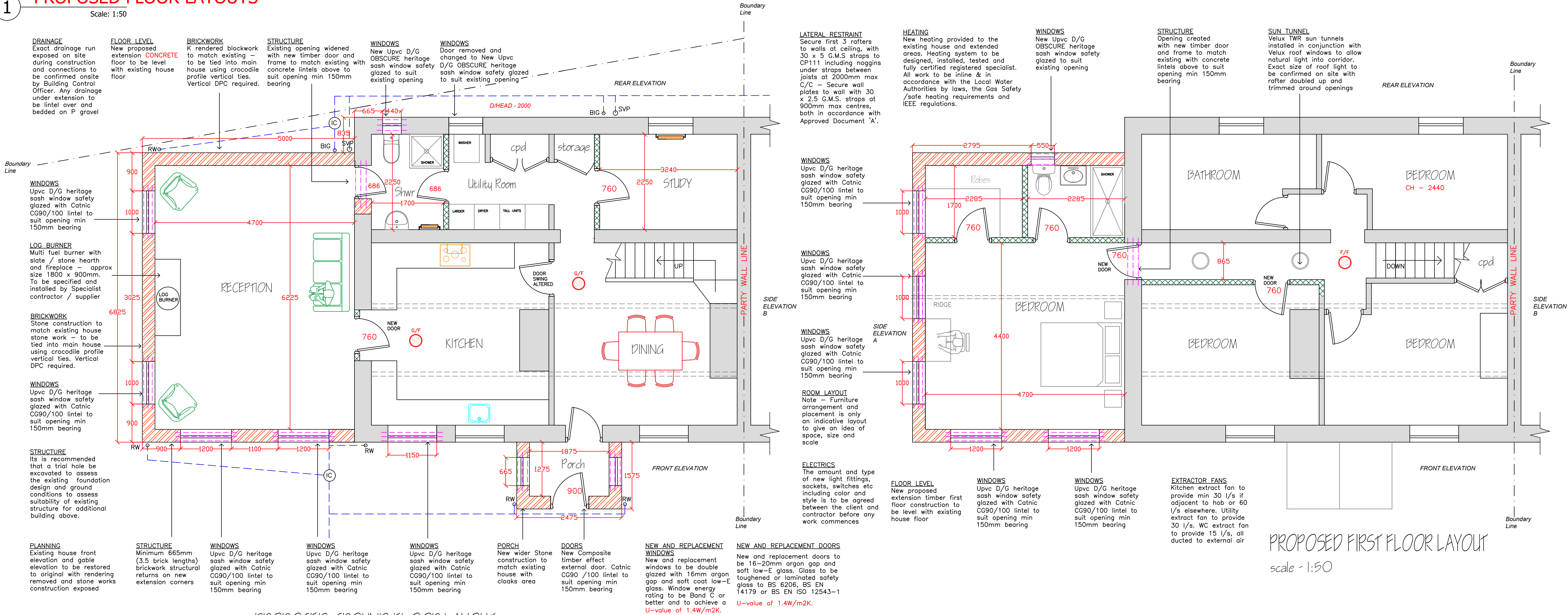
PROPOSED GROUND FLOOR LAYOUT scale - 1:50
