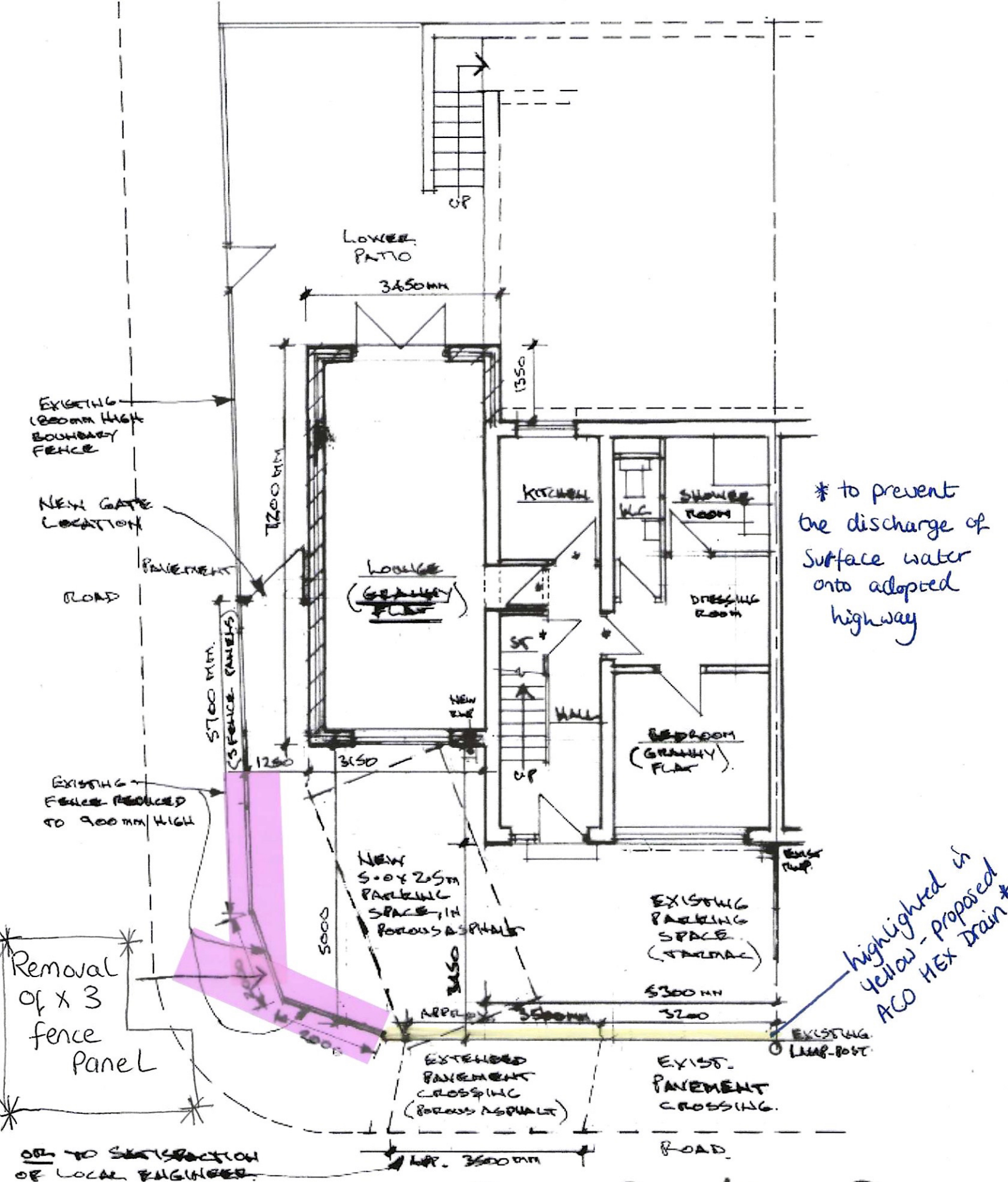
GROUND FLOOR PLAN/SITE PLAN
