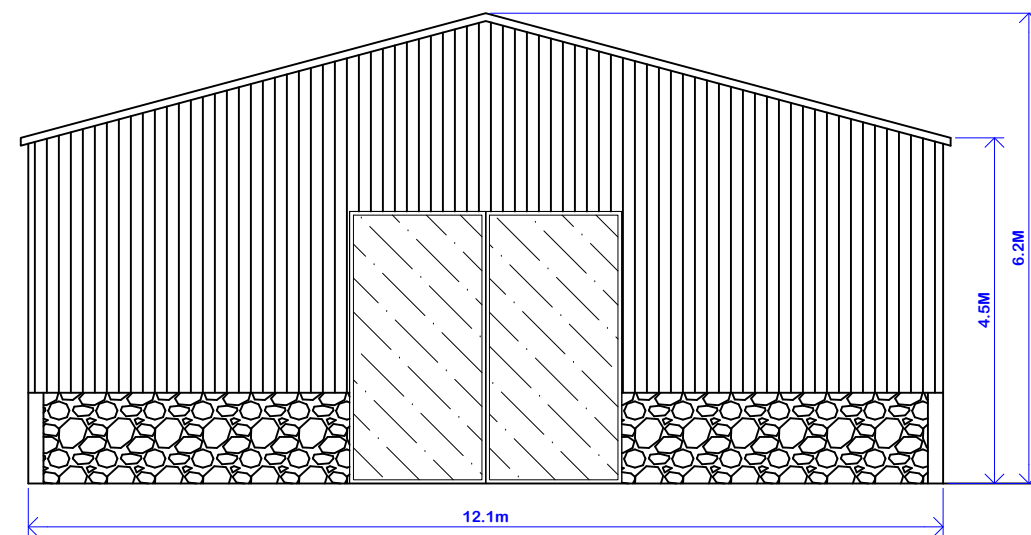
PROPOSED SOUTH FACING ELEVATION
