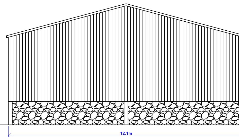
PROPOSED SOUTH FACING ELEVATION
